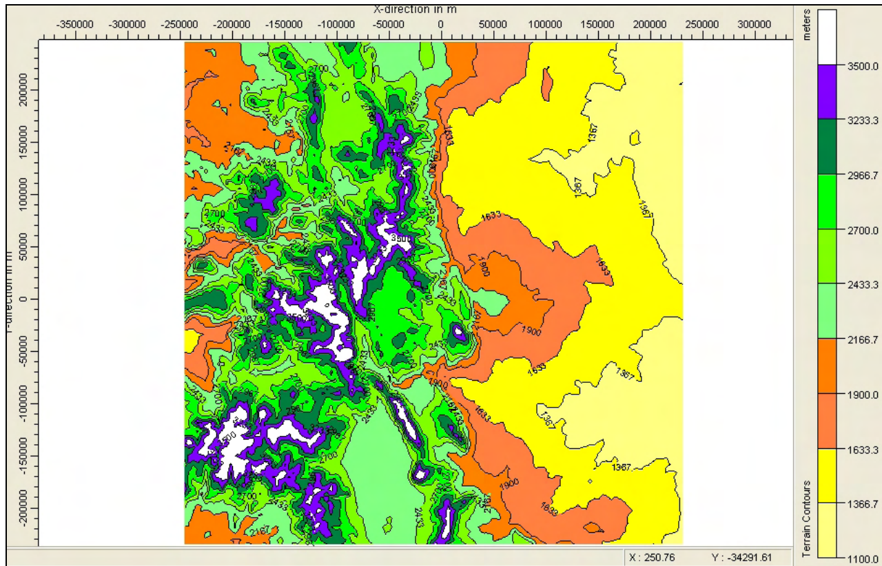
Figure 2. CALMET Terrain.
