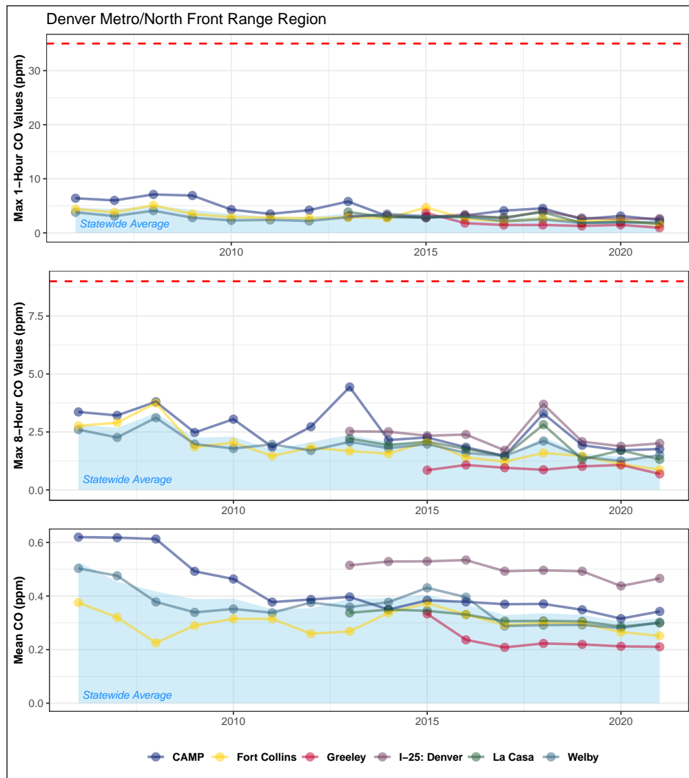
Figure 4.9: Fifteen-year trend in annual maximum one-hour (top) and eight-hour (center) CO values and annual mean eight-hour CO concentrations (bottom) for monitoring sites in the Denver Metro/Northern Front Range region. The one-hour and eight-hour NAAQS (35 ppm and 9 ppm, respectively) are shown as dashed red lines.
