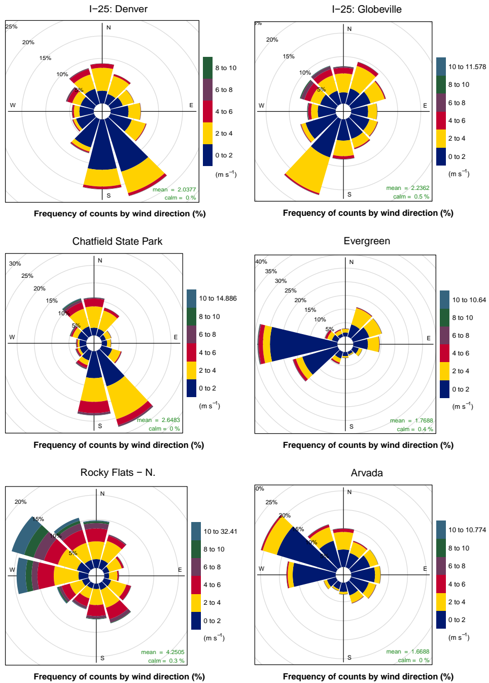
Figure 4.26: Wind roses for sites in the Denver Metro/North Front Range Region during 2021 (continued).
