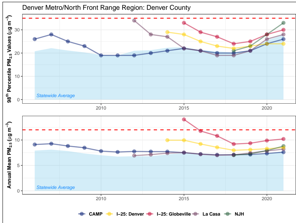
Figure 4.5: Fifteen-year trend in 24-hour PM 2.5 annual 98 th percentile values (top) and annual mean concentrations (bottom) for monitoring sites in Denver County. The 24-hour and annual mean NAAQS (35 µg m -3 and 12 µg m -3 , respectively) are shown as dashed red lines.
