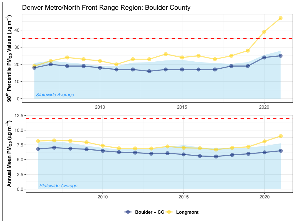
Figure 4.4: Fifteen-year trend in 24-hour PM 2.5 annual 98 th percentile values (top) and annual mean concentrations (bottom) for monitoring sites in Boulder County. The 24-hour and annual mean NAAQS (35 µg m -3 and 12 µg m -3 , respectively) are shown as dashed red lines.
