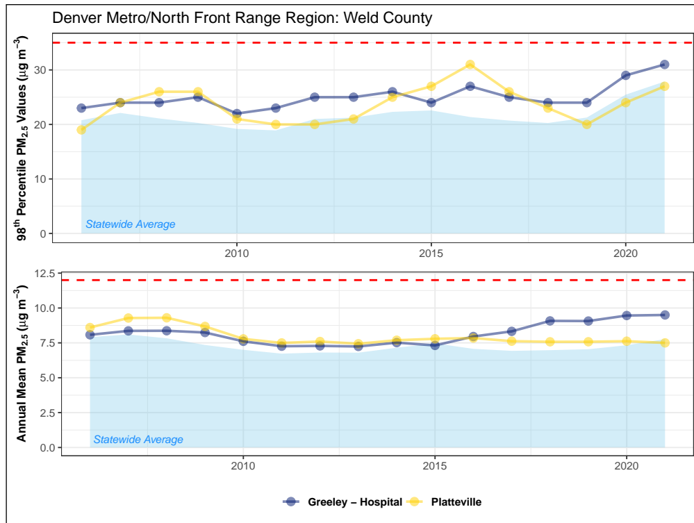
Figure 4.8: Fifteen-year trend in 24-hour PM 2.5 annual 98 th percentile values (top) and annual mean concentrations (bottom) for monitoring sites in Weld County. The 24-hour and annual mean NAAQS (35 µg m -3 and 12 µg m -3 , respectively) are shown as dashed red lines.
