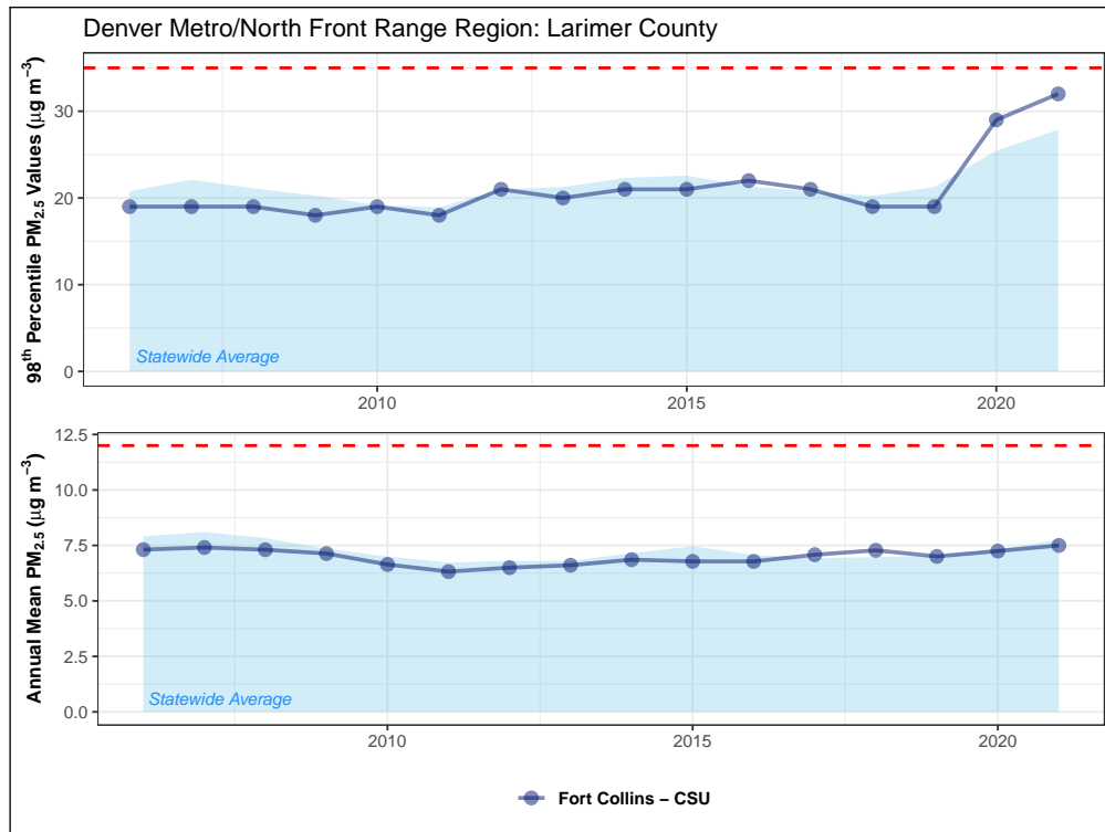
Figure 4.7: Fifteen-year trend in 24-hour PM 2.5 annual 98 th percentile values (top) and annual mean concentrations (bottom) for monitoring sites in Larimer County. The 24-hour and annual mean NAAQS (35 µg m -3 and 12 µg m -3 , respectively) are shown as dashed red lines.
