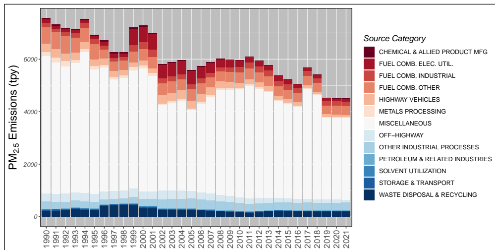
Figure 2.19: Trends in national PM 2.5 emissions from 1990 to 2021.
