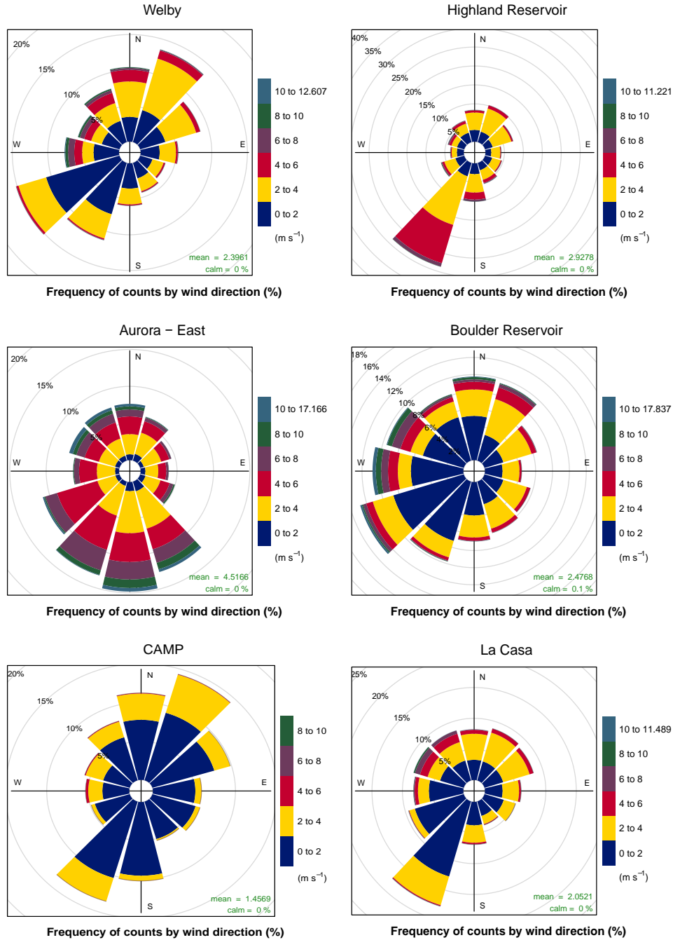
Figure 4.25: Wind roses for sites in the Denver Metro/North Front Range Region during 2021.
