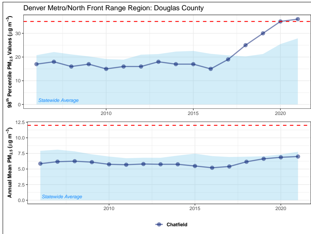
Figure 4.6: Fifteen-year trend in 24-hour PM 2.5 annual 98 th percentile values (top) and annual mean concentrations (bottom) for monitoring sites in Douglas County. The 24-hour and annual mean NAAQS (35 µg m -3 and 12 µg m -3 , respectively) are shown as dashed red lines.
