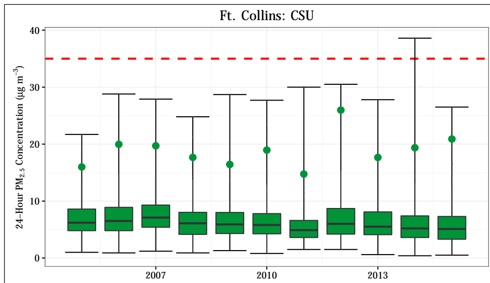
Figure 4.19: 24-hr PM 2.5 concentrations at the Ft. Collins - CSU station. The 24-hour standard (35 µg m -3 ) is shown as a dashed red line. The annual design value (98 th percentile of values measured throughout the year) is shown for each year as a green point.
