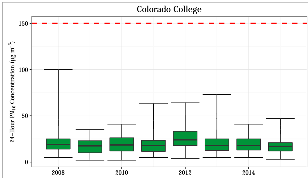
Figure 4.52: 24-hour average PM 10 concentrations at the Colorado College station. The 24-hour standard (150 µg m -3 ) is shown as a dashed red line.
