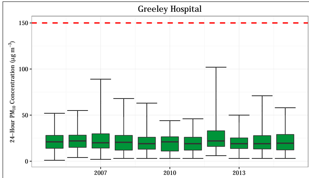
Figure 4.20: 24-hr PM 10 concentrations at the Greeley - Hospital station. The 24-hour standard (150 µg m -3 ) is shown as a dashed red line.
