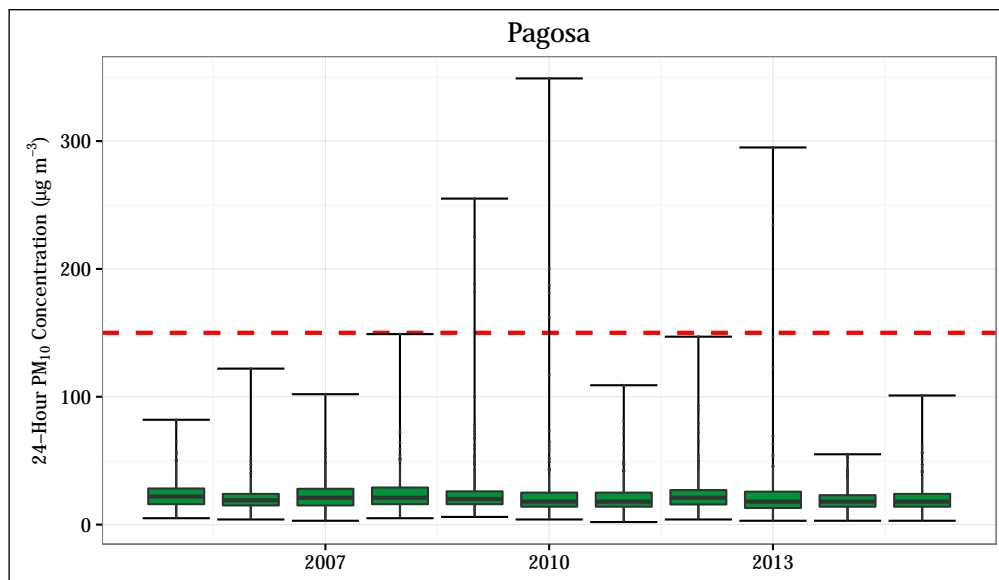
Figure 4.64: 24-hour average PM 10 concentrations at the Pagosa Springs School station. The 24-hour standard (150 µg m -3 ) is shown as a dashed red line.
