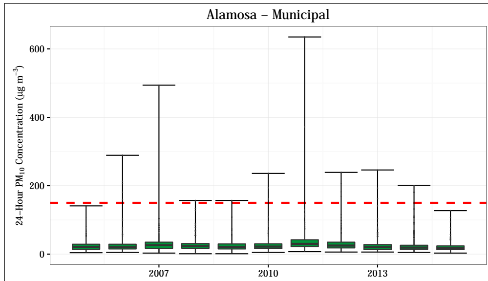
Figure 4.61: 24-hour average PM 10 concentrations at the Alamosa - Municipal station. The 24-hour standard (150 µg m -3 ) is shown as a dashed red line.
