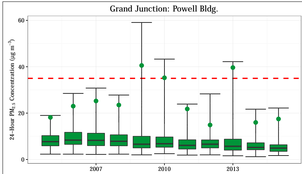
Figure 4.73: 24-hr PM 2.5 concentrations at the Grand Junction - Powell Bldg. station. The 24-hour standard (35 µg m -3 ) is shown as a dashed red line. The annual design value (98 th percentile of values measured throughout the year) is shown for each year as a green point.
