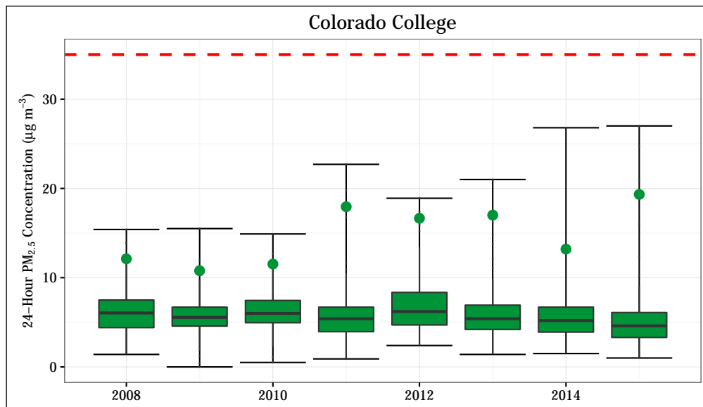
Figure 4.53: 24-hr PM 2.5 concentrations at the Colorado College station. The 24-hour standard (35 µg m -3 ) is shown as a dashed red line. The annual design value (98 th percentile of values measured throughout the year) is shown for each year as a green point.
