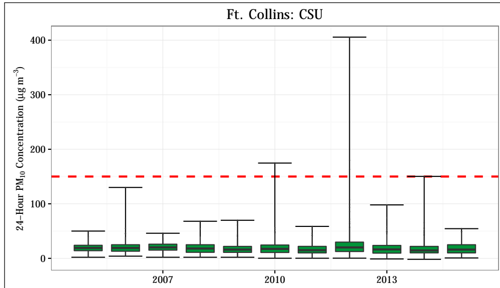
Figure 4.18: 24-hr PM 10 concentrations at the Ft. Collins - CSU station. The 24-hour standard (150 µg m -3 ) is shown as a dashed red line.
