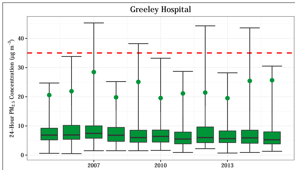
Figure 4.21: 24-hr PM 2.5 concentrations at the Greeley - Hospital station. The 24-hour standard (35 µg m -3 ) is shown as a dashed red line. The annual design value (98 th percentile of values measured throughout the year) is shown for each year as a green point.
