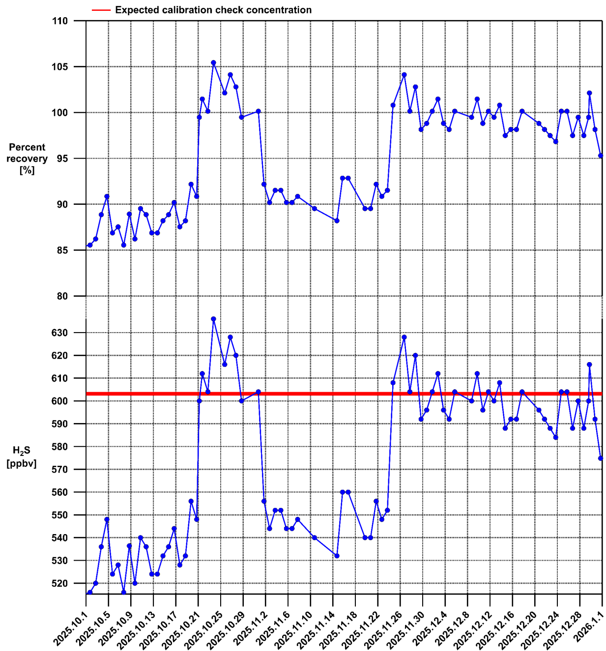
Figure 11. Time series of hydrogen sulfide ( \text{H}_2\text{S} ) automated calibration checks for the Teledyne Model T101 \text{H}_2\text{S} analyzer at the Adams County Birch Street site during 2025 Q4.
