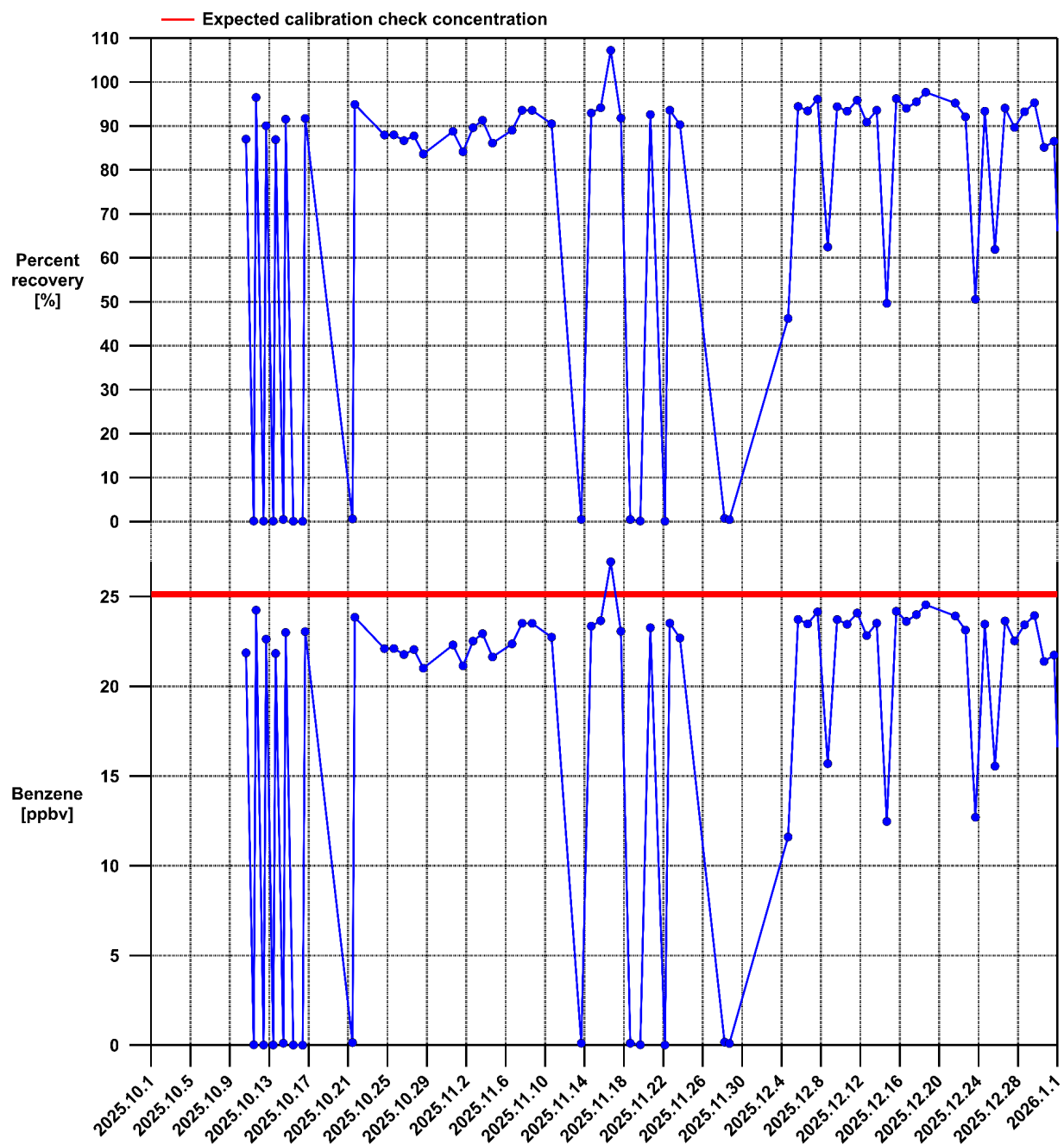
Figure 10. Time series of benzene ( C_6H_6 ) automated calibration checks for the Dual-Cavity AROMA-TOX instrument at the Adams County Birch Street site during 2025 Q4.
