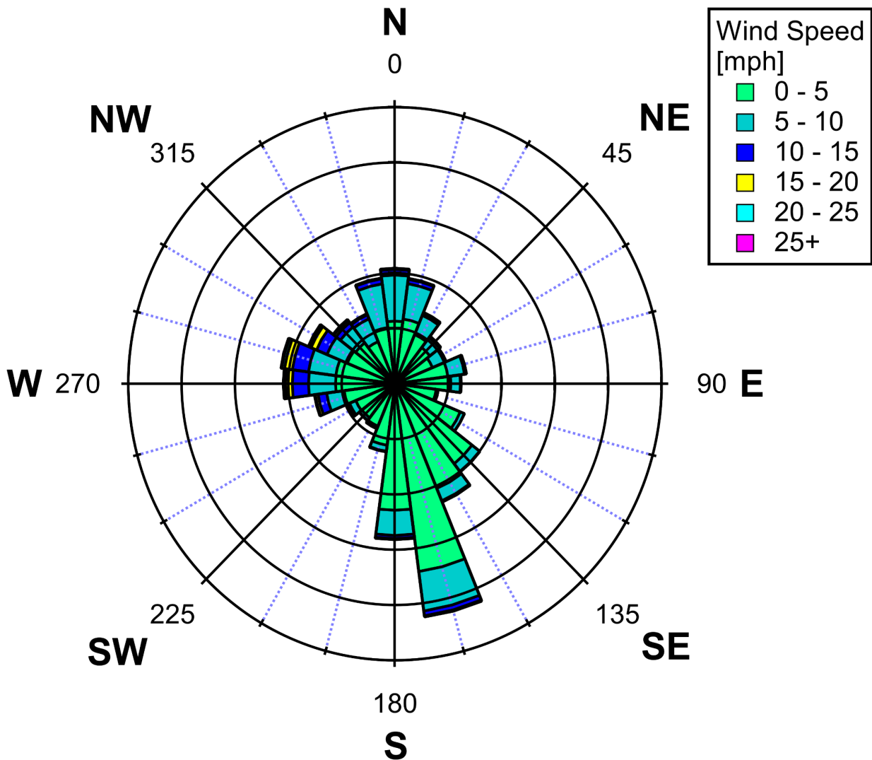
Figure 4. Wind rose measured by the MT GOAT network at the Adams County Birch Street site during 2025 Q4. The colored wedges indicate the direction that the wind is coming from.
