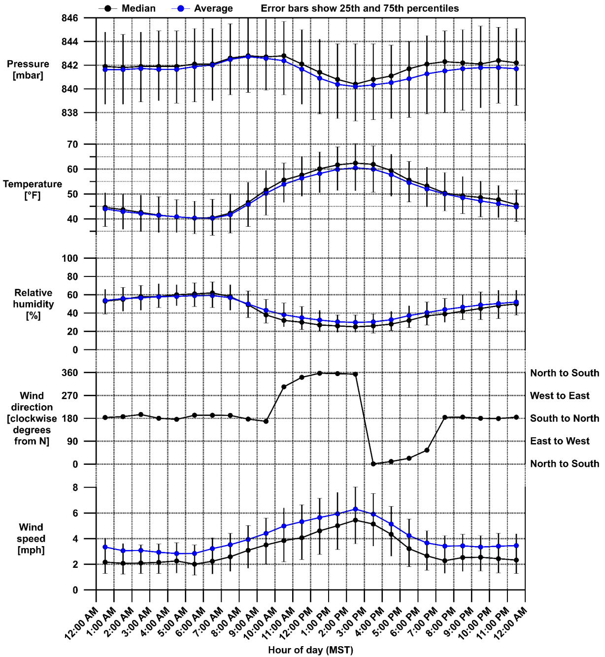
Figure 9. Diurnal plot for pressure, temperature, relative humidity, wind direction, and wind speed measured by the MT GOAT site at the Adams County Birch Street site during 2025 Q4.
