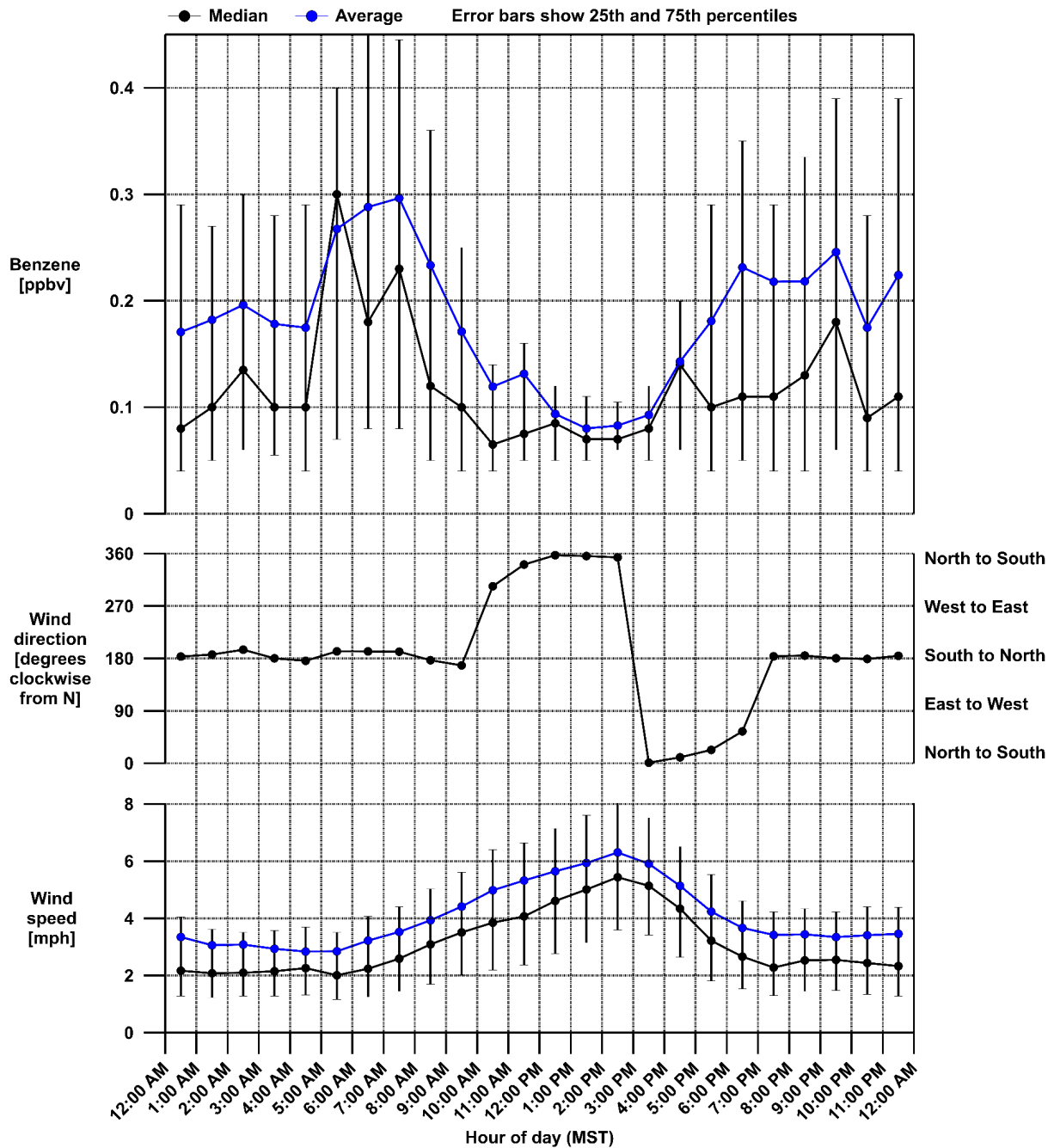
Figure 7. Diurnal plot for benzene ( C_6H_6 ), wind speed, and wind direction measured by the MT GOAT site at the Adams County Birch Street site during 2025 Q4.
