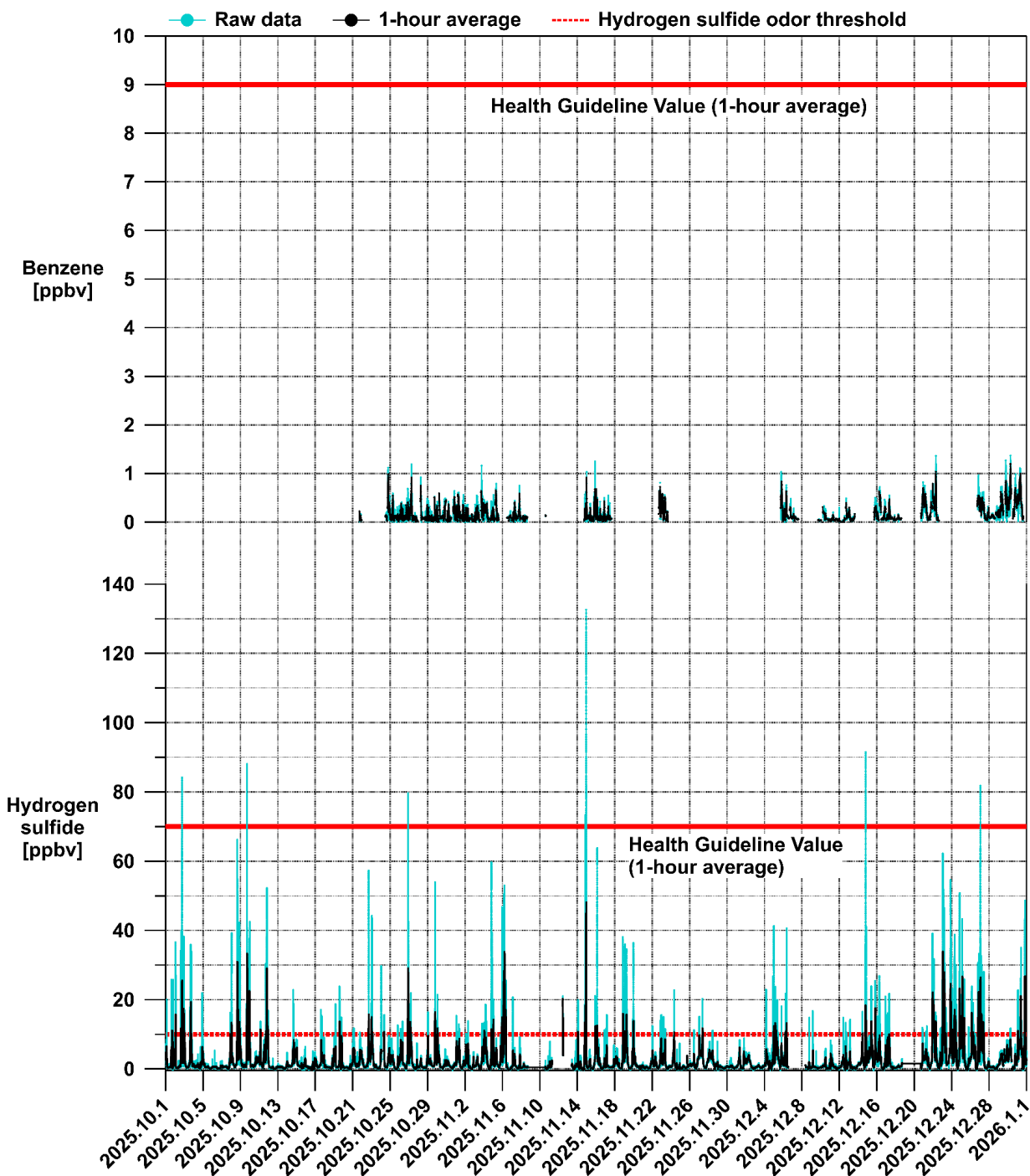
Figure 2. Time series of benzene ( C_6H_6 ) and hydrogen sulfide ( H_2S ) concentrations measured by the MT GOAT network at the Adams County Birch Street site during 2025 Q4. The measured benzene ( C_6H_6 ) concentration is compared to the Health Guideline Value (HGV) of 9 ppbv for a one-hour average. The measured hydrogen sulfide ( H_2S ) concentration is compared to the Health Guideline Value (HGV) of 70 ppbv for a one-hour average. The hydrogen sulfide ( H_2S ) typical odor threshold of 10 ppbv is also shown.
