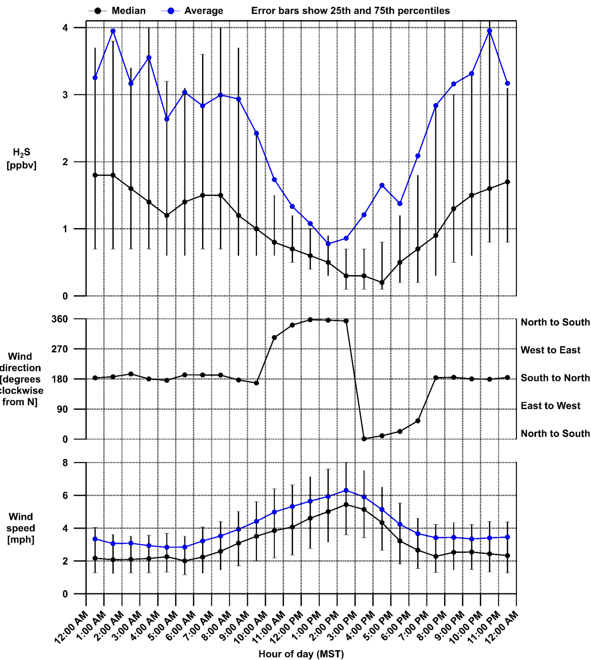
Figure 8. Diurnal plot for hydrogen sulfide (H 2 S), wind speed, and wind direction measured by the MT GOAT site at the Adams County Birch Street site during 2025 Q4.
