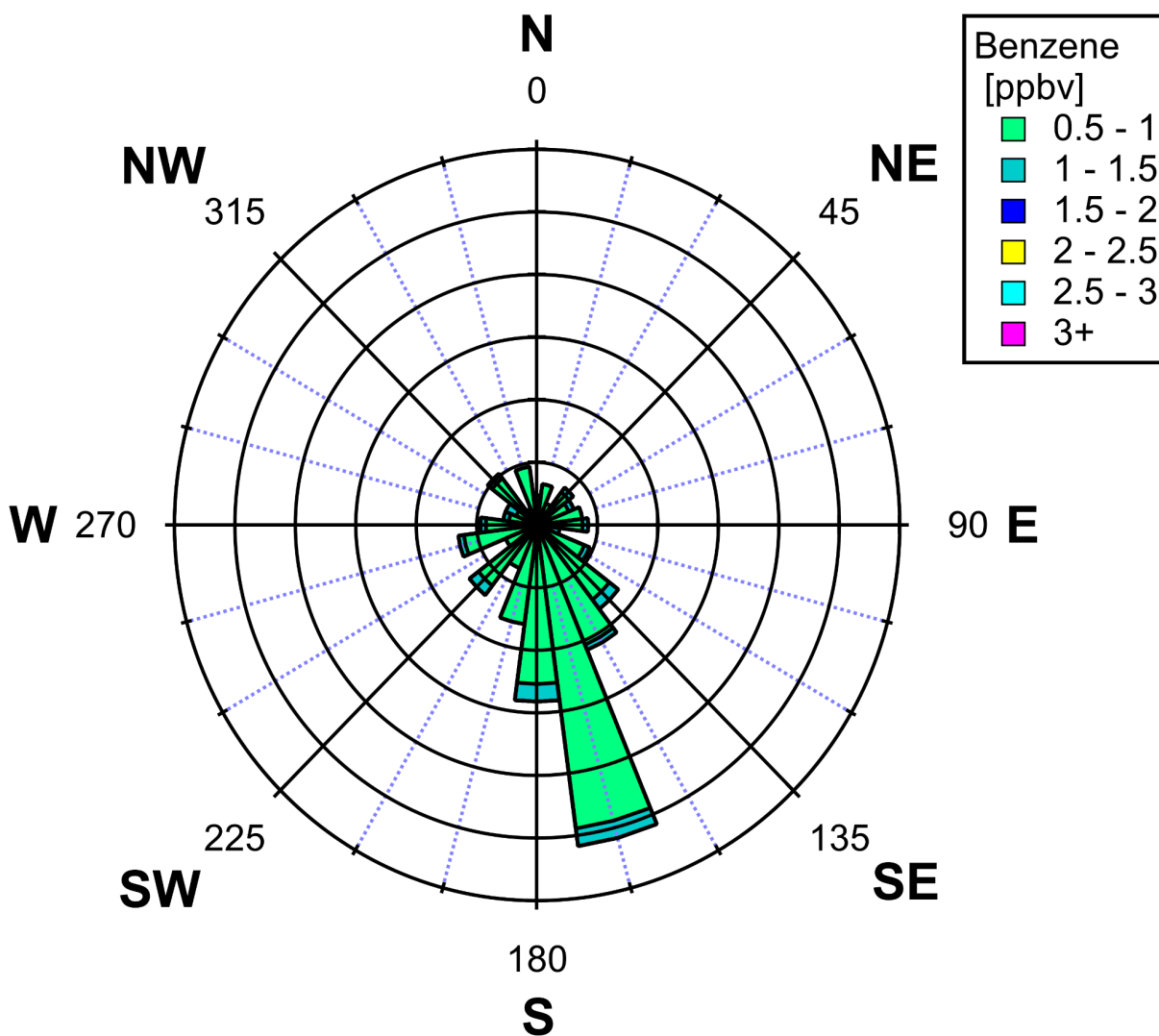
Figure 5. Pollution rose for benzene ( C_6H_6 ) measured by the MT GOAT network at the Adams County Birch Street site during 2025 Q4. Benzene ( C_6H_6 ) concentrations below 0.5 ppbv are excluded from the pollution rose.
