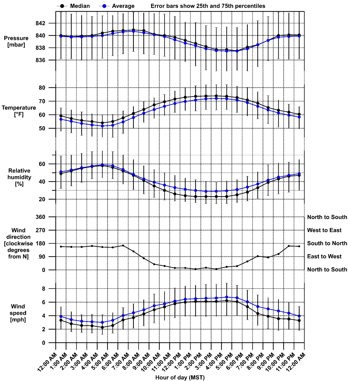
Figure 7. Diurnal plot for pressure, temperature, relative humidity, wind direction, and wind speed measured by the MT GOAT network at the Adams County Birch Street site during 2026 Q2.
