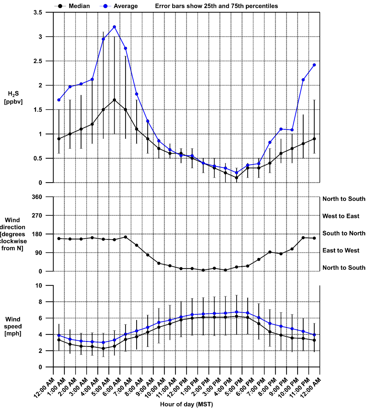
Figure 6. Diurnal plot for hydrogen sulfide ( H_2S ), wind speed, and wind direction measured by the MT GOAT network at the Adams County Birch Street site during 2026 Q2.
