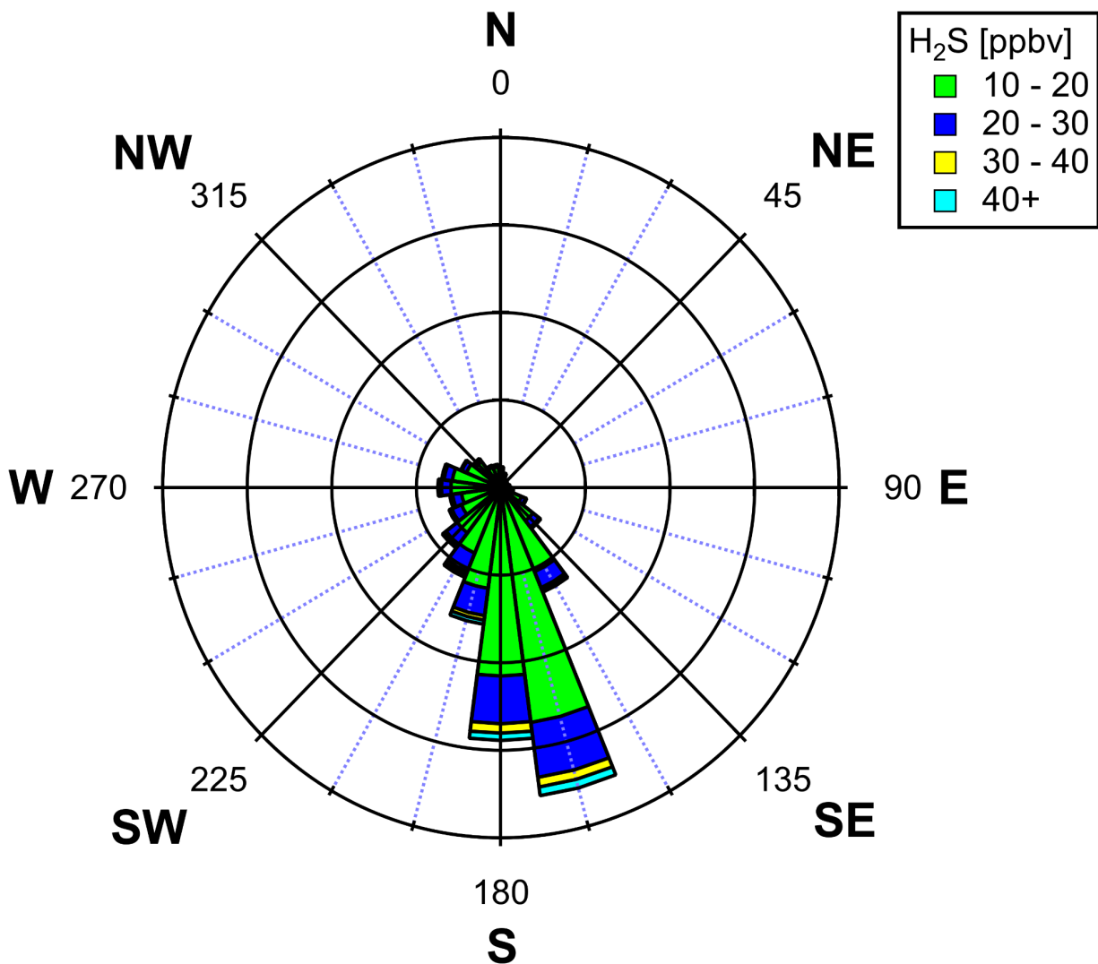
Figure 5. Pollution rose for hydrogen sulfide (H 2 S) measured by the MT GOAT network at the Adams County Birch Street site during 2026 Q2. Hydrogen sulfide (H 2 S) concentrations below 10 ppbv are excluded from the pollution rose.
