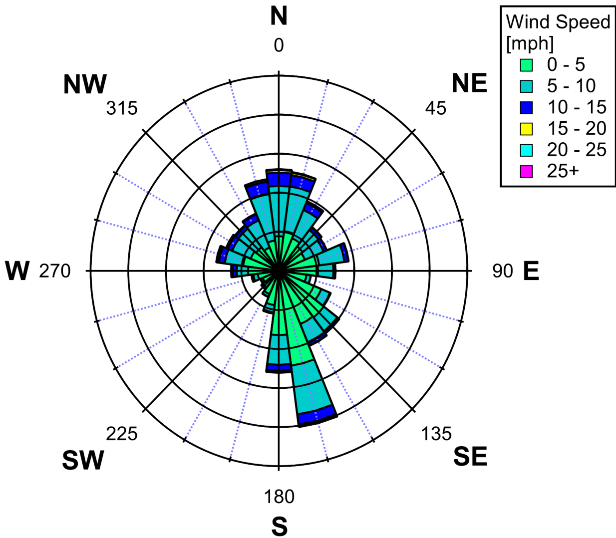
Figure 4. Wind rose measured by the MT GOAT network at the Adams County Birch Street site during 2026 Q2. The colored wedges indicate the direction that the wind is coming from.
