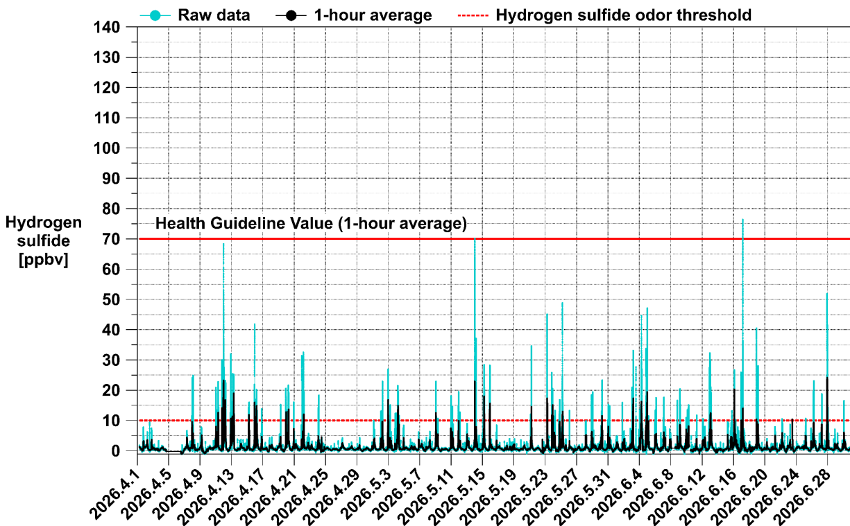
Figure 2. Time series of hydrogen sulfide ( \text{H}_2\text{S} ) concentrations measured by the MT GOAT network at the Adams County Birch Street site during 2026 Q2. The measured hydrogen sulfide ( \text{H}_2\text{S} ) concentration is compared to the Health Guideline Value (HGV) of 70 ppbv for a one-hour average. The hydrogen sulfide ( \text{H}_2\text{S} ) typical odor threshold of 10 ppbv is also shown.
