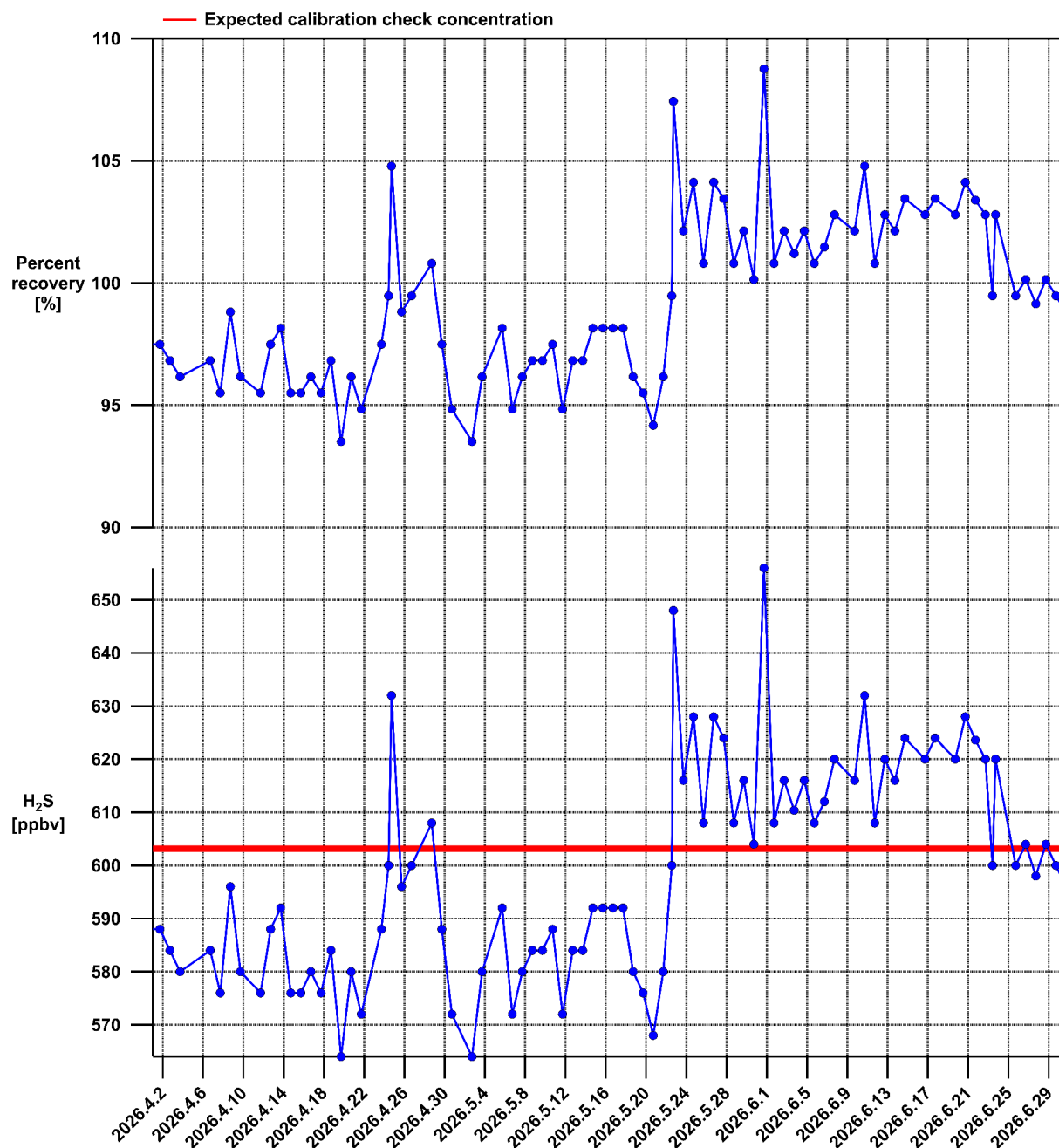
Figure 11. Time series of hydrogen sulfide (H 2 S) automated calibration checks for the Teledyne Model T101 H 2 S analyzer at the Adams County Birch Street site during 2026 Q2.
