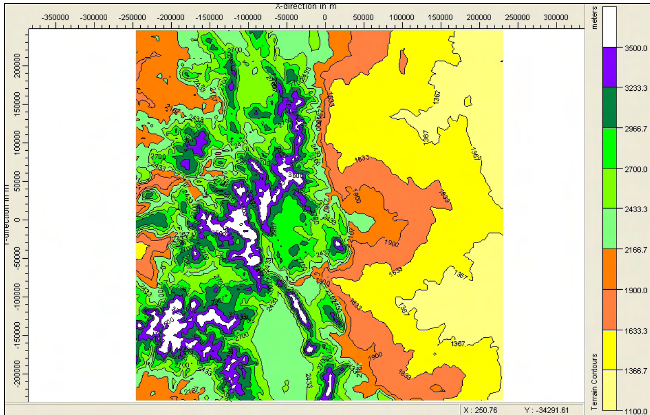
Figure 2. CALMET Terrain.
