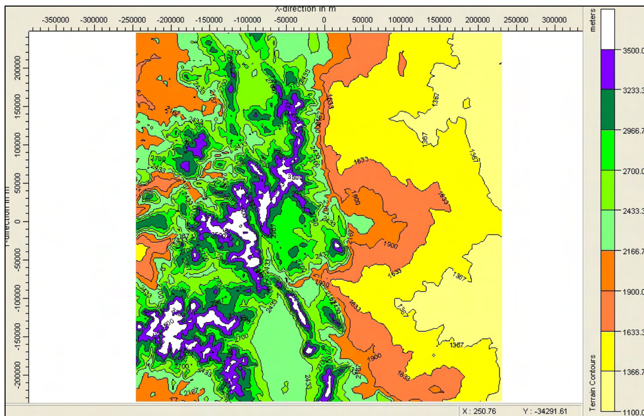
Figure 2. CALMET Terrain.
